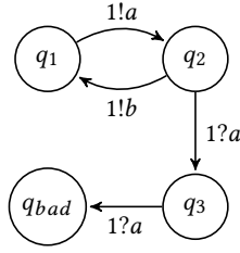
Figure 1: Simple example of a lossy channel system.
