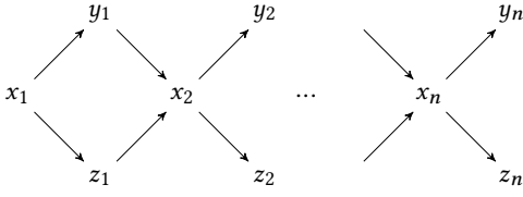
Figure 5: MOF for the language L of Example 6.2.
