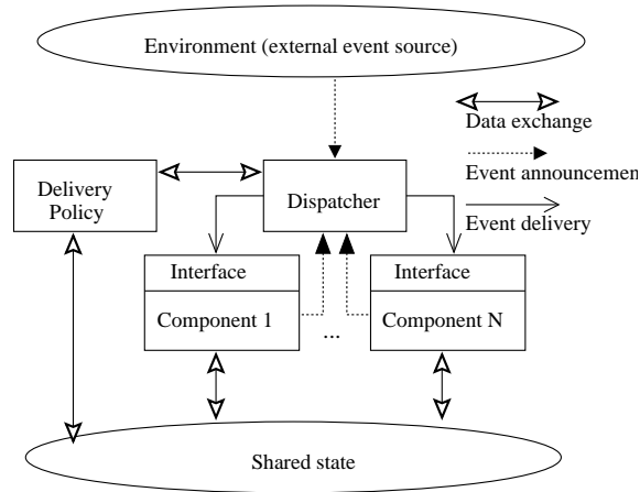
Fig. 1. Structure of a Pub-Sub System Model
