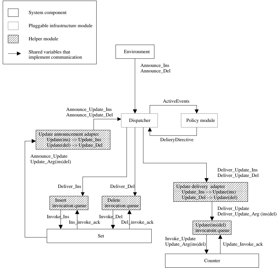
Fig. 4. Generated Set-and-Counter Model
