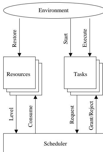
Fig. 5. Mobile Resource Allocation System
