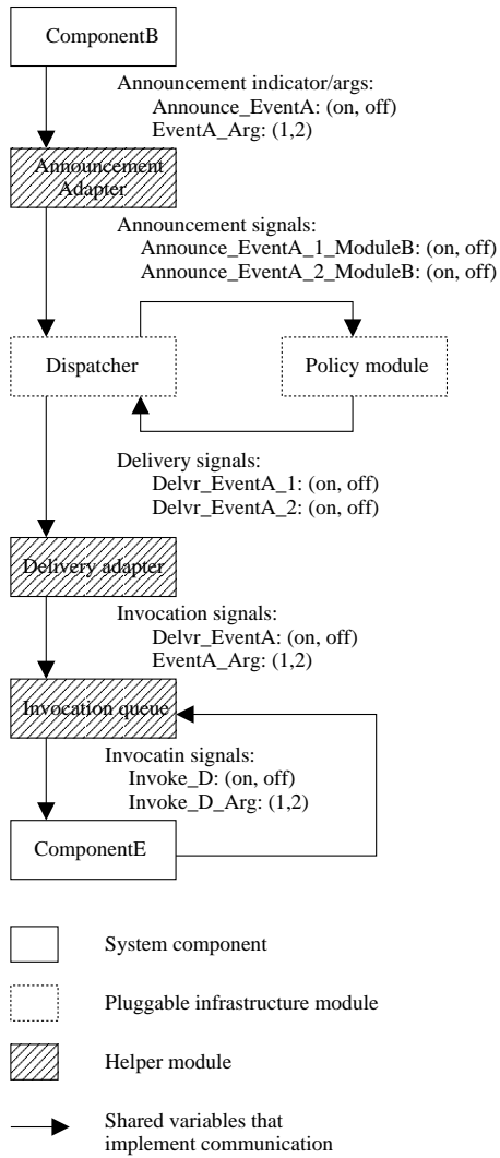
Fig. 3. Event Dispatch Structures
